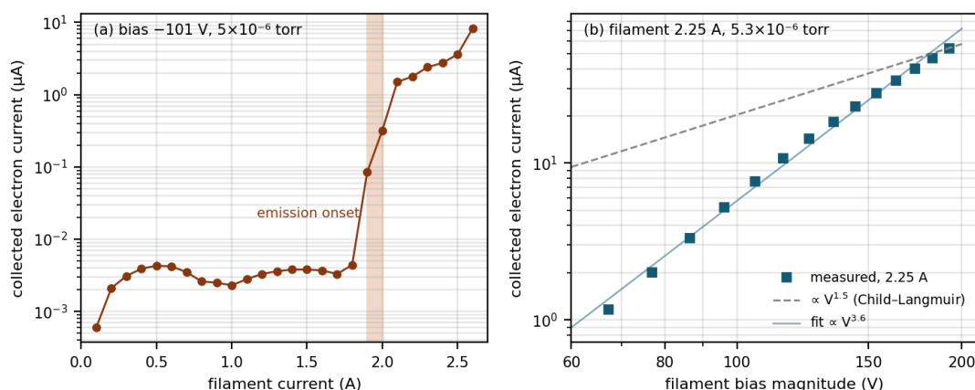
Figure 7. Filament bench data from the design workbook, 2018. (a) Collected electron current against filament current at -101 V, showing the sharp onset between 1.8 and 2.0 A. (b) Collected current against bias magnitude at 2.25 A, with the V^{1.5} Child-Langmuir slope the workbook tabulated against and a power-law fit to the data.
