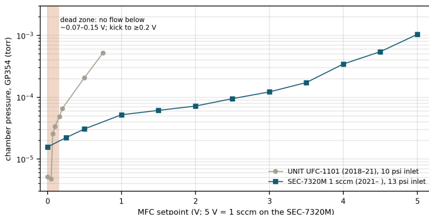
Figure 9. Mass-flow-controller setpoint against chamber pressure for the two controllers (design workbook, sheet "MFC flow"; ion-gauge readings, hydrogen-corrected where gas was flowing). The shaded band is the dead zone. The UNIT unit's series stops at 0.75 V because above that only the rough gauge read.
